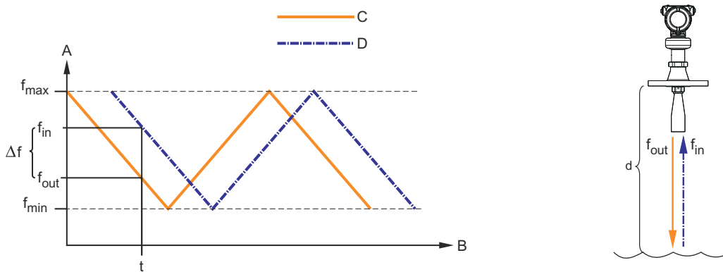
Figure 1: FMCW-method
