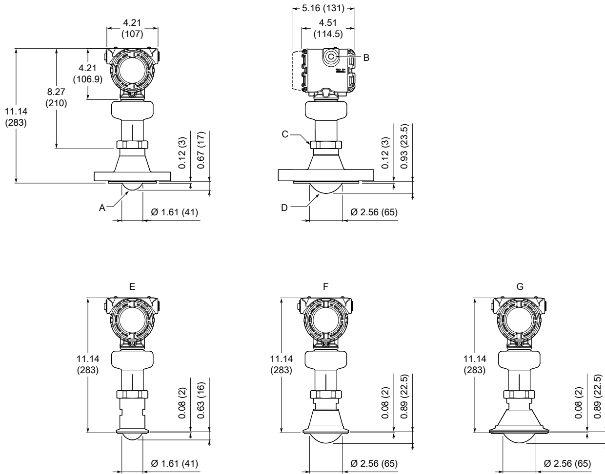
Figure 23: Process Seal Antenna
