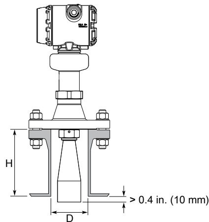
Figure 15: Mounting of the Cone Antenna
