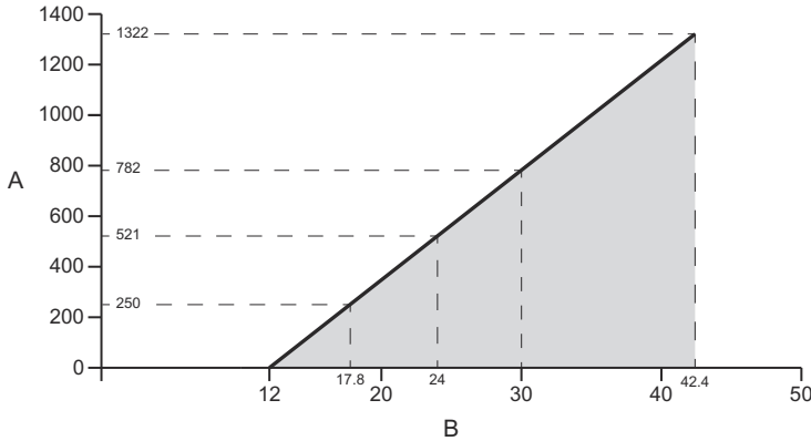
Figure 5: Load Limits
