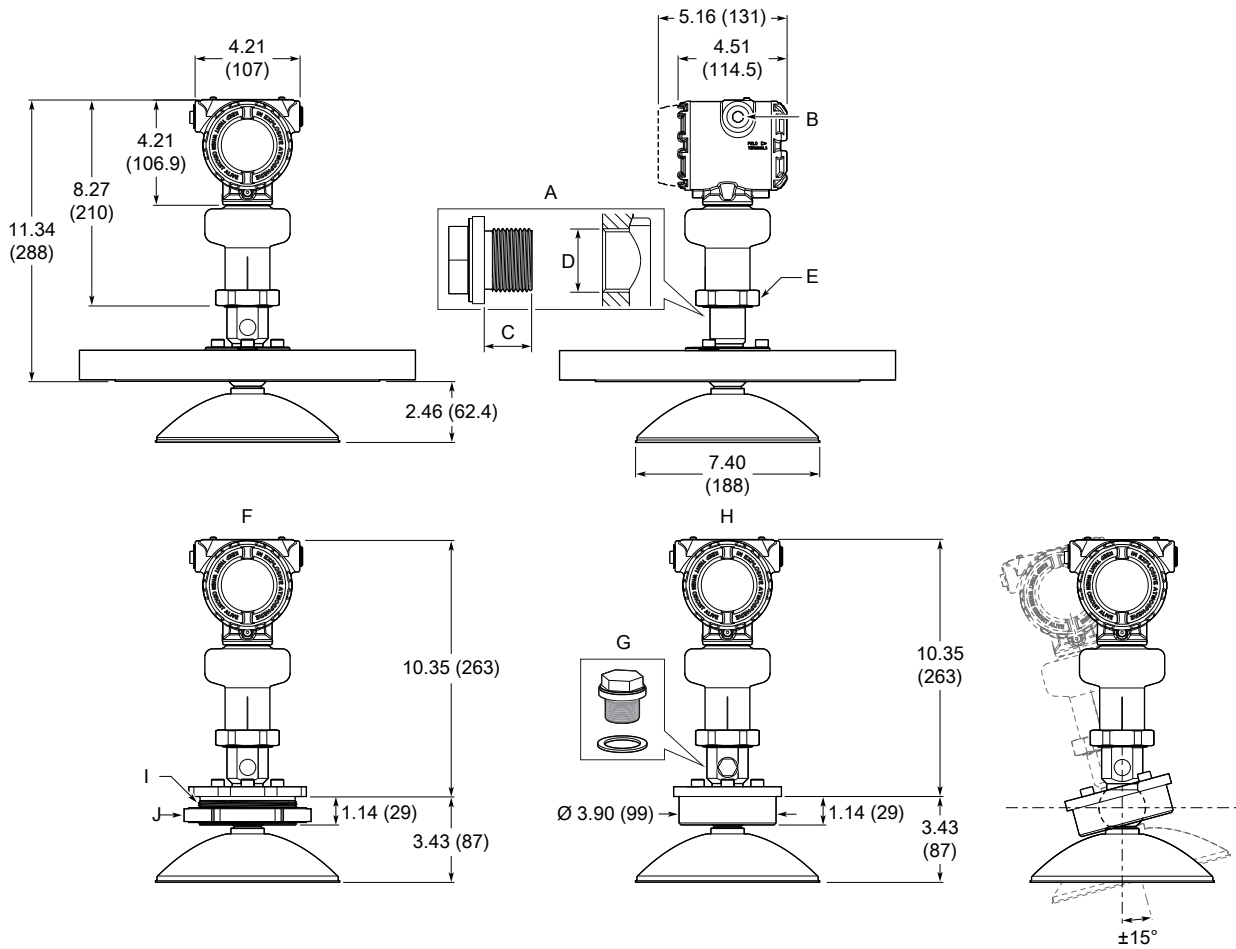
Figure 24: Parabolic Antenna
