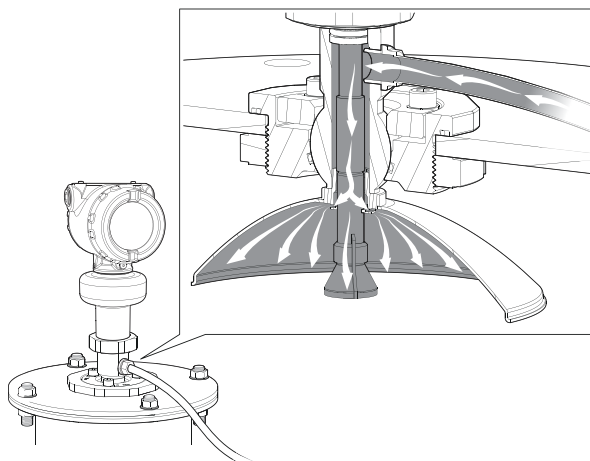
Figure 11: Air Purging for Parabolic Antenna
