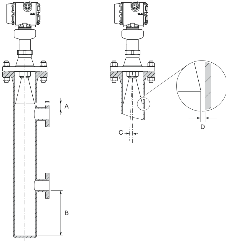
Figure 19: Chamber Requirements
