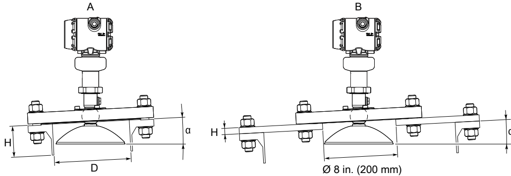
Figure 17: Mounting of the Parabolic Antenna
