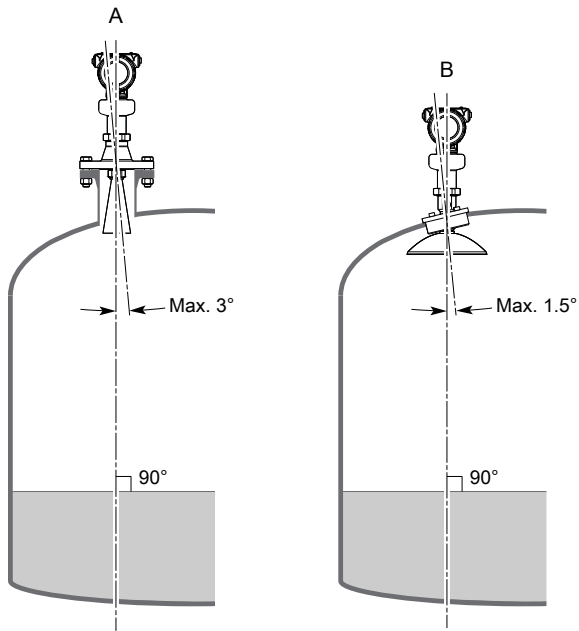
Figure 14: Inclination
