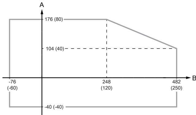
Figure 10: Ambient Temperature vs. Process Temperature
